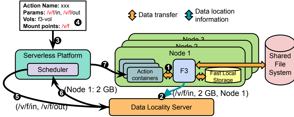
Figure 5.2: CNSBench architecture and locality-aware data operations
