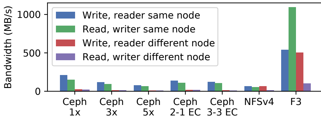
Figure 5.7: Comparison of read-while-write performance, when readers and writers are on the same or different nodes. For CephFS, having the reader and writer on different nodes significantly degrades both read and write performance. MinIO is absent from this experiment due to its inability to read and write data concurrently. F3 was layered on top of an unreplicated CephFS volume.
