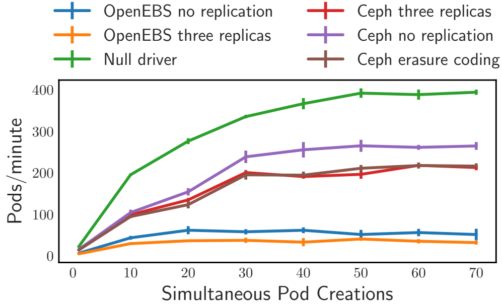
Figure 4.5: Volume creations and attachments per minute, for different numbers of simultaneous operations. The vertical lines at each point shows the standard deviation for volume creation and attachment rate at that point.
