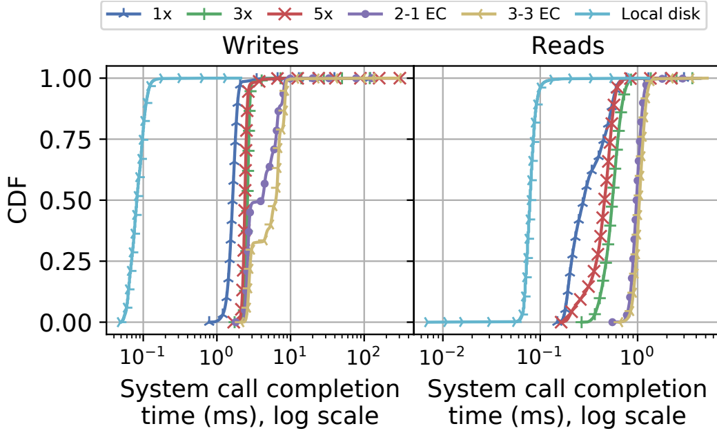
Figure 5.4: CDFs of read and write system call latencies, for different storage configurations. We used log scale for the x-axis because the system calls exhibited long tails at higher replication degrees.
