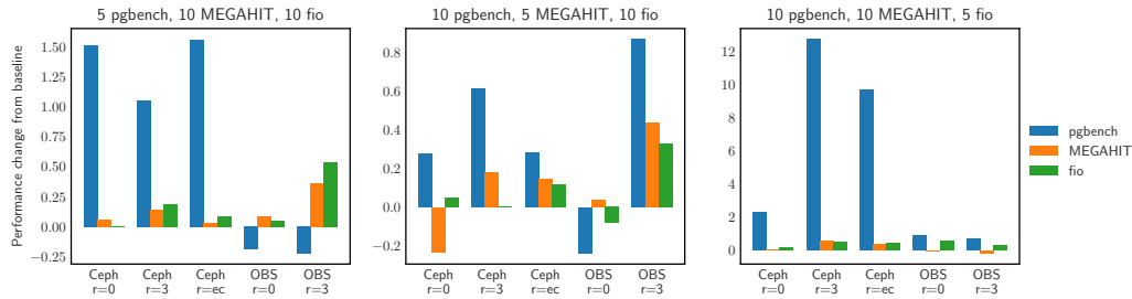
Figure 4.8: Change in performance compared to baseline, for three different ratios of I/O workload on five different storage configurations.
