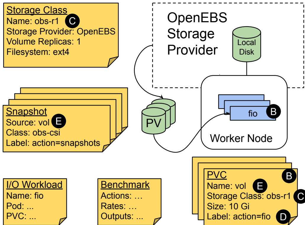
Figure 4.3: Subset of a Kubernetes cluster with a single worker node and a PV. Shows the CNSBench resources that are involved (the I/O Workload and Benchmark), as well as the core Kubernetes resources created by the CNSBench controller according to the Benchmark specification (the Snapshots, PVCs, PV, and workload Pods).
