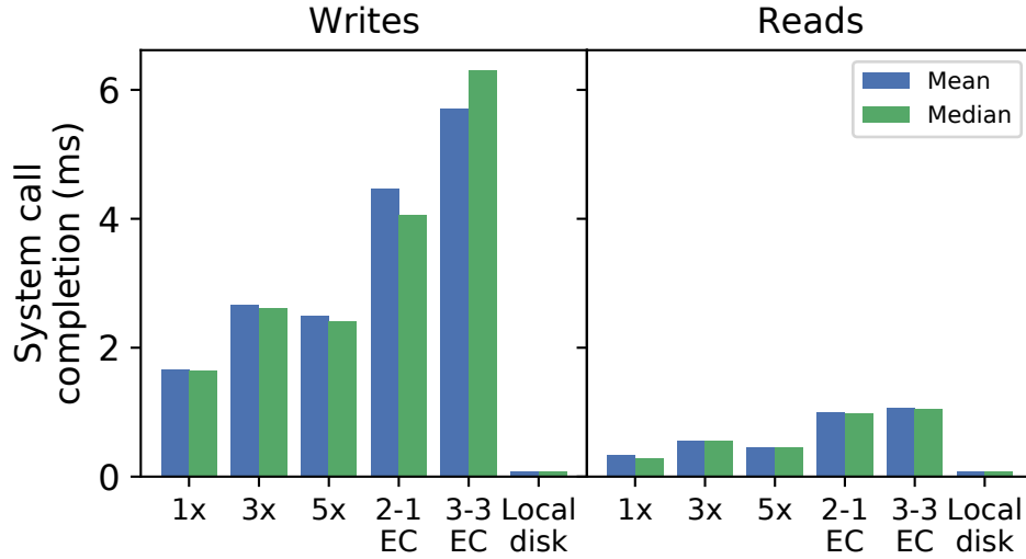
Figure 5.3: Mean and median system call latencies for different configurations of storage system. 1\times , 3\times , and 5\times refer to the degree of replication; 2-1 and 3-3 EC refer to the erasure coding configuration (2 data and 1 coding chunk, and 3 data and 3 coding chunks, respectively).
