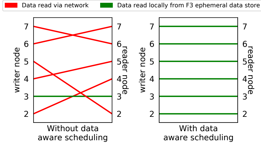
Figure 5.5: Impact of data aware scheduling. Each line connects a writer with its corresponding reader, with the numbers along each side showing what node in the cluster the writer or reader ran on. Red lines indicate that the reader needed to transfer its file from the writer node via a network transfer. Green lines indicate that the reader and writer ran on the same node and the file was read from F3’s local ephemeral data store, with no network transfer was needed.
