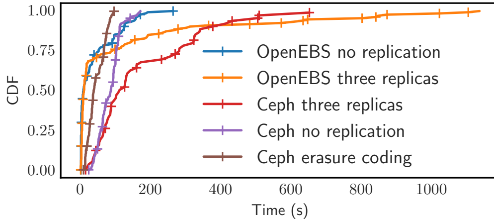
Figure 4.7: CDF of snapshot creation times for different storage provider configurations.
