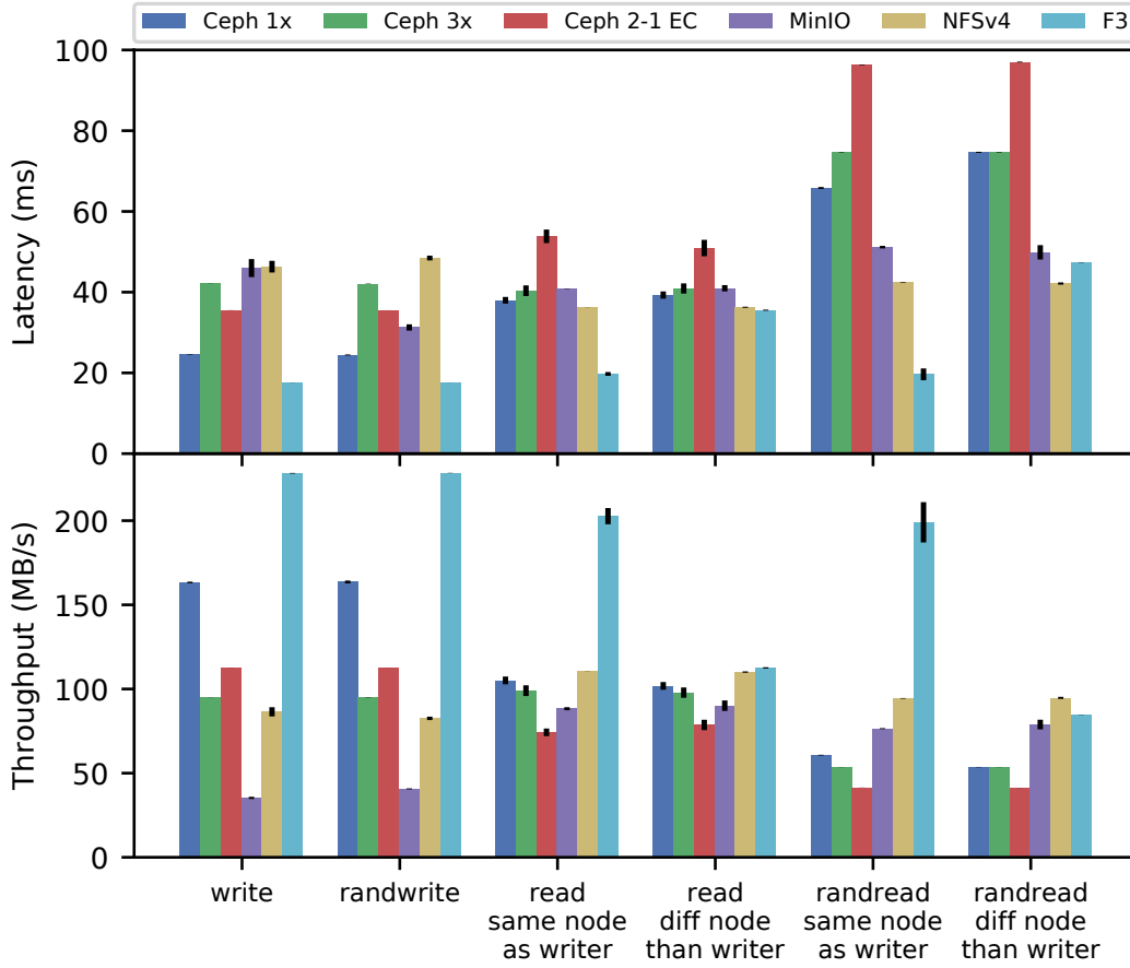
Figure 5.6: Mean latencies and bandwidths of Ceph, NFS, MinIO, and F3. “Ceph 1×” and “Ceph 3×” are configured with 1× and 3× replication, respectively. “Ceph 2-1 EC” uses erasure coding (data split into two data chunks and one coding chunk). F3 was layered on top of an unreplicated CephFS volume.
