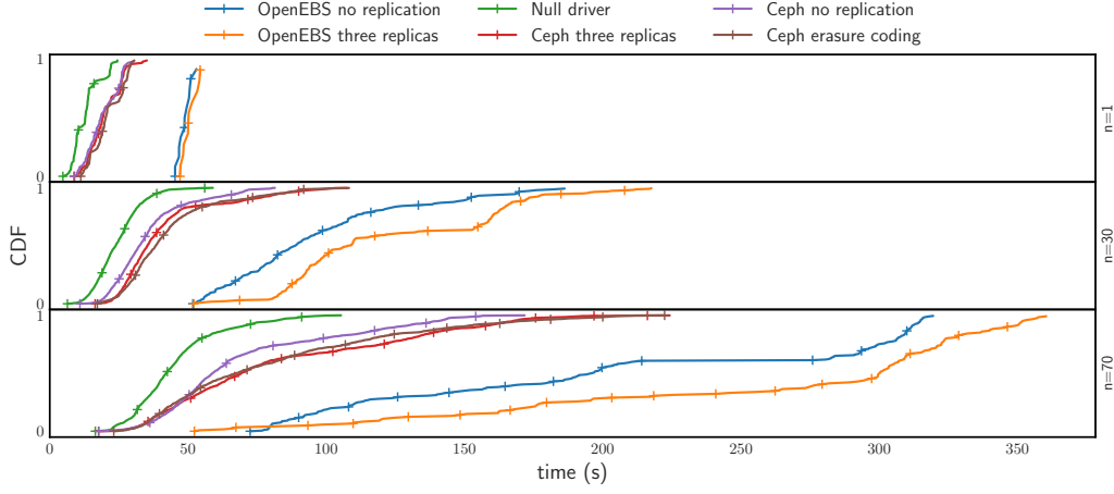
Figure 4.4: CDFs of time required to create and attach volumes for different storage provider configurations. n is the number of simultaneous volume creations. For all storage configurations, increasing the number of simultaneous volume operations increased the average time to create and attach an individual volume.
