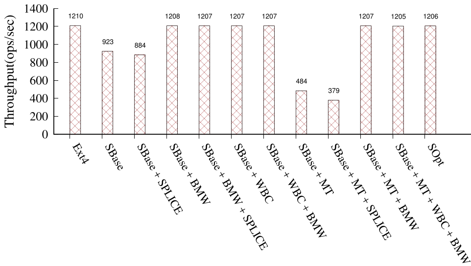
Fig. 14. Impact of incremental optimizations on throughput on HDD SEQ-WR-128KB-1TH-1F.
