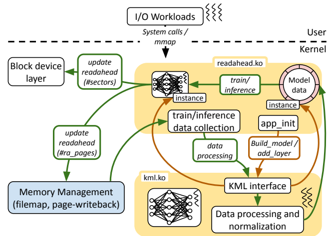
Figure 1: Kernel space training/inference architecture.
