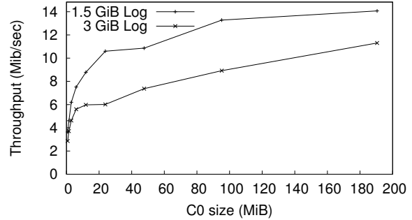
Figure 7: Performance of Story Book’s Fable backend with varying in-memory tree component sizes.
