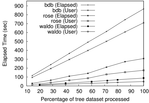
Figure 6: Performance of Waldo and Story Book’s insert tool on logs of different sizes.
