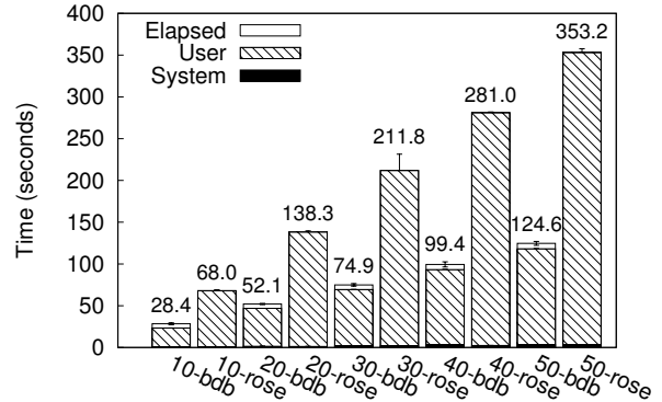
Figure 9: Performance of a provenance query.
